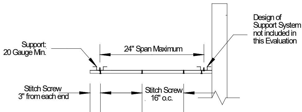
TYPICAL ASSEMBLY SECTION VIEW
